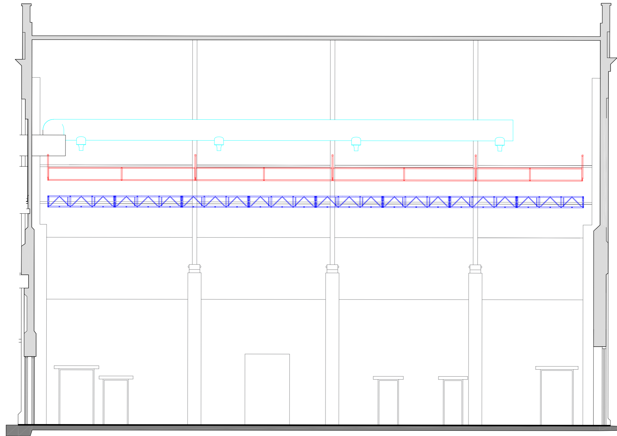
CC SIDE SECTION - Looking East
